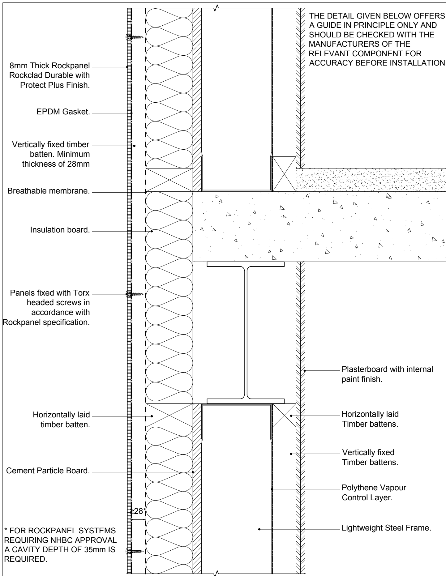
DETAIL 16 - ROCKCLAD DURABLE WITH PROTECT PLUS FINISH VERTICAL SECTION TIMBER SUBSTRUCTURE TO STRUCTURAL STEEL WITH LIGHT STEEL FRAME.
